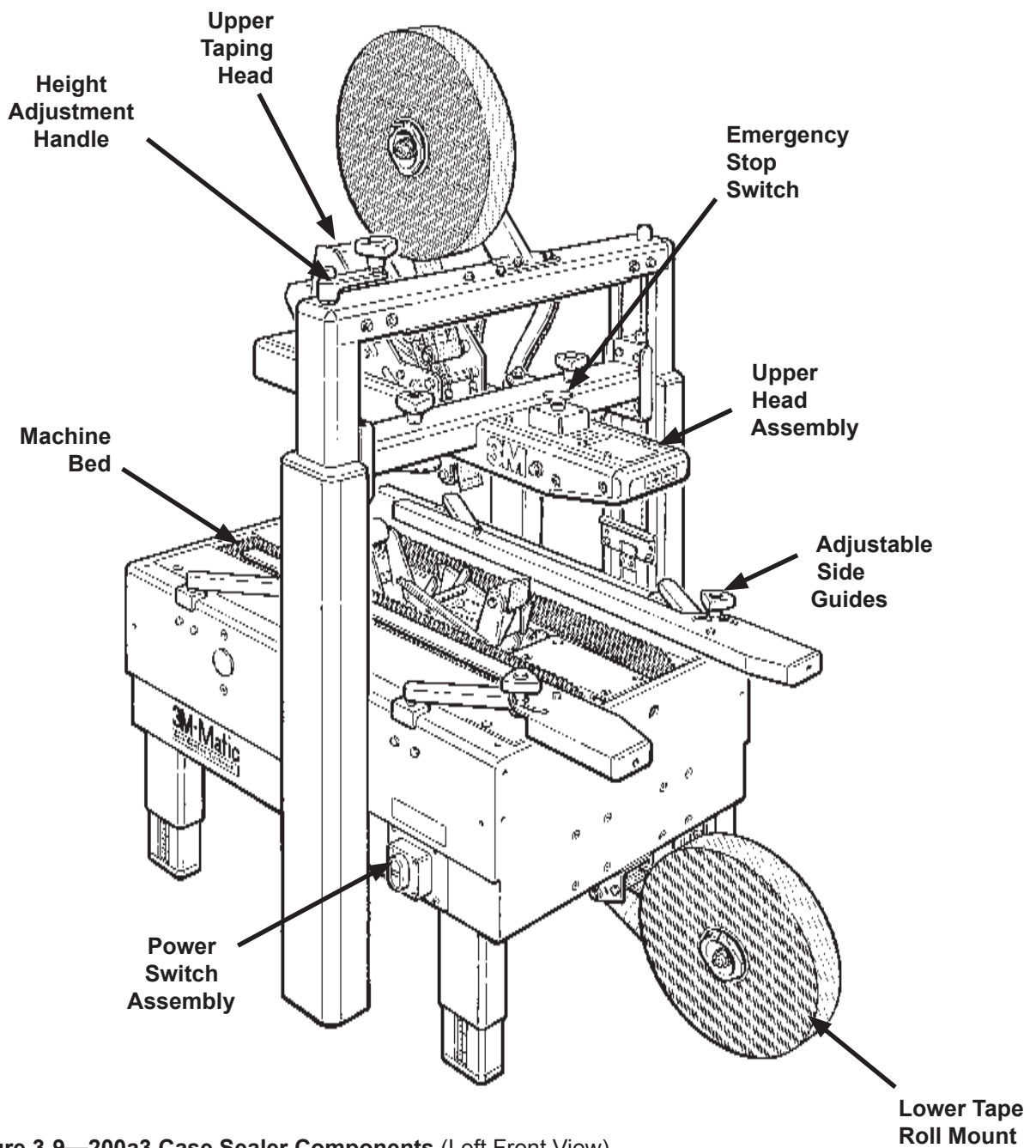
Figure 3-9—200a3 Case Sealer Components (Left Front View)
